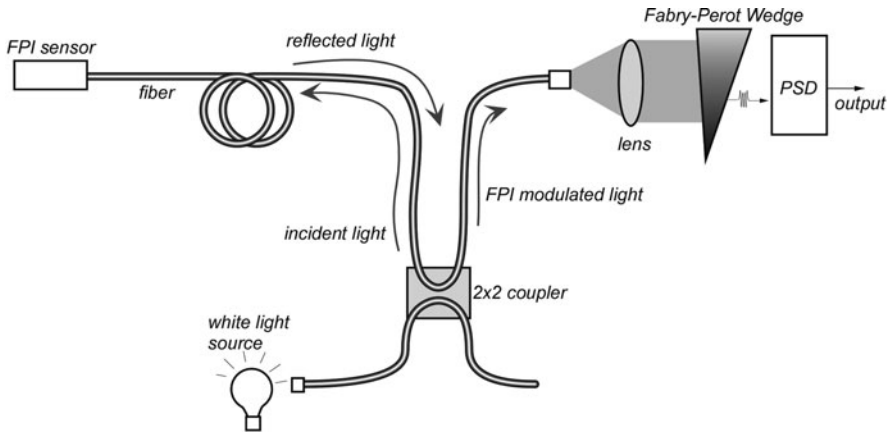
Fig. 7.35 Measuring system for the Fabry-Perot sensor (courtesy of Roctest. www.roctest.com )
