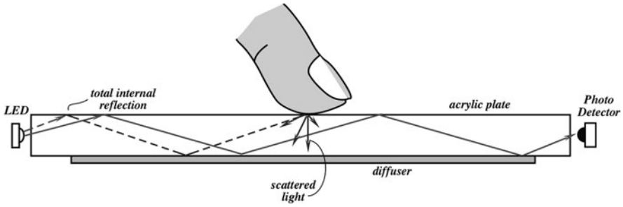
Fig. 9.17 Concept of optical touch screen
