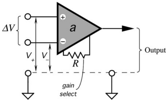
Fig. 5.8 Instrumentation amplifier
