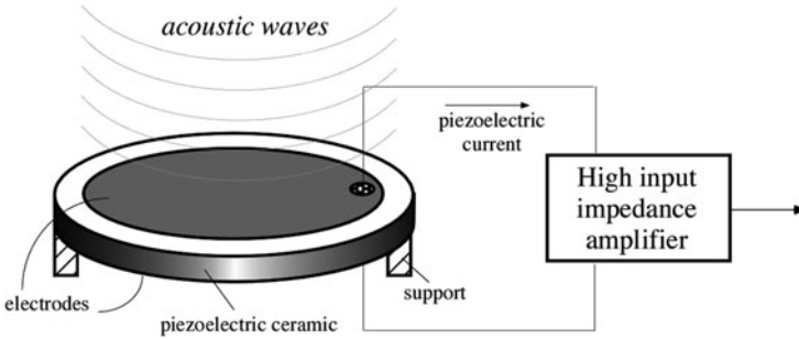
Fig. 12.4 Piezoelectric microphone
