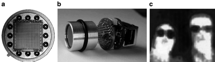
Fig. 14.21 Thermopile thermal-imaging sensor: sensing surface (a); imaging module (b); and example of a thermal image (c) (courtesy of Heimann Sensors, www.heimannsensors.com )
