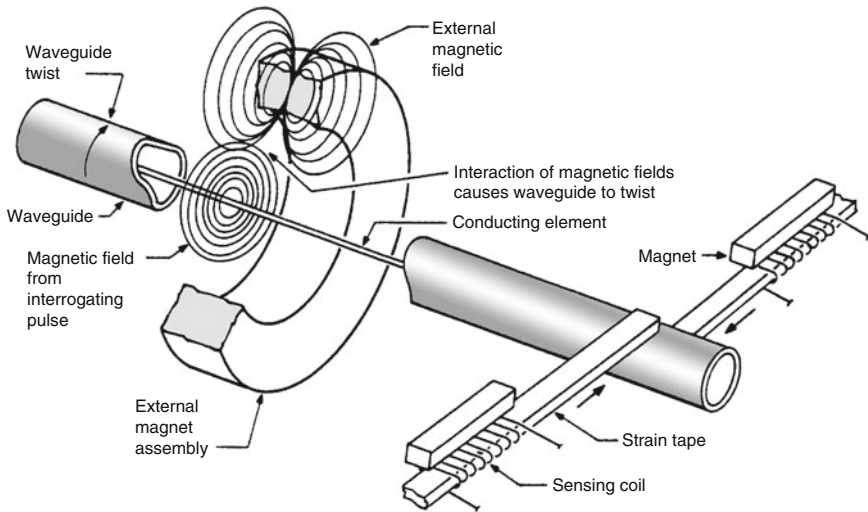
Fig. 7.27 A magnetostrictive detector uses ultrasonic waves to detect position of a permanent magnet
