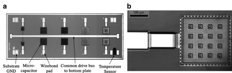
Fig 17.8 MEMS chip (2 \times 5 mm) containing a variety of parallel-plate capacitor designs (a). Close-up top-view of a parallel-plate capacitor (b)
