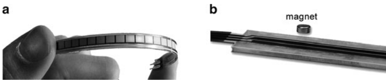
Fig. 7.5 Flex sensor (a) and MagnetoPot (b) (courtesy of spectrasymbol.com)
