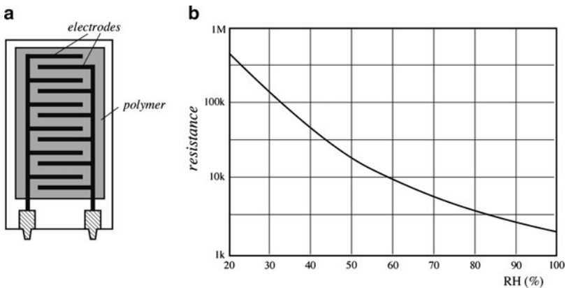
Fig. 3.20 Hygriстора design (a) and its transfer function (b)
