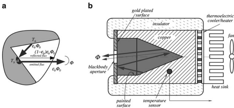
Fig. 3.46 Cavity effect enhances emissivity (a); construction of a practical blackbody with a dual cavity surface (b)
