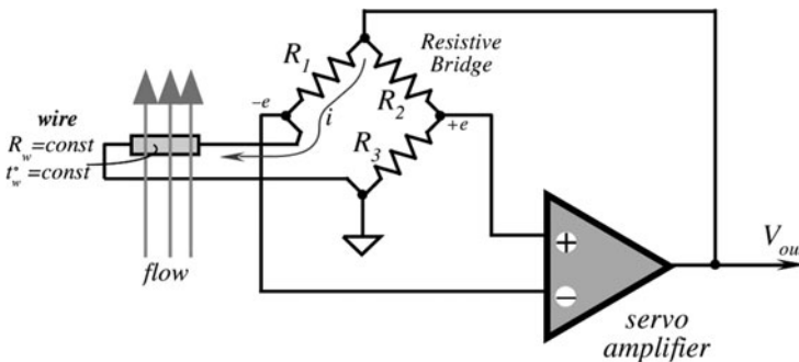
Fig. 11.5 Null-balancing bridge for a constant temperature hot-wire anemometer
