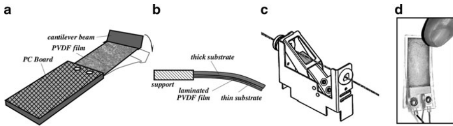
Fig. 9.6 PVDF film switch for a pinball machine (a), beam switch (b), thread break sensor (c) (from [6]), laminated tactile sensor (d)
